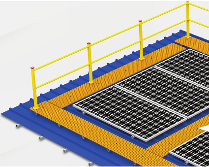
FRP Handrail Assembly
